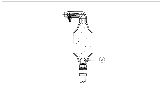
fig. 7.2.5 - The air accumulated inside the body pushes the rubber ball (2) to the bottom, thus blocking the passage. At this point the valve closes and the rubber ball prevents the air accumulated inside the body of the air supply unit from reaching the pump intake.
