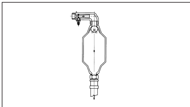
fig. 7.2.3 - When the pump starts up, the intake pressure is lower than the pressure in the surge tank. This difference causes water to flow from the surge tank to the pump intake, through the air supply unit.
