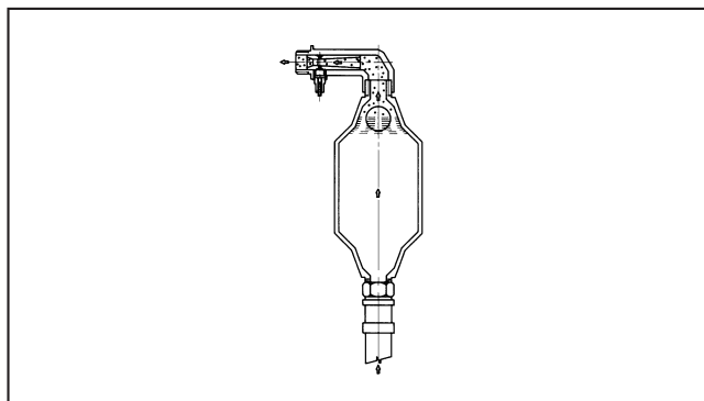
fig. 7.2.6 - When the pump stops the depression ceases and a flow of water is produced, which lifts the ball and pushes the air in the body of the supply unit into the tank.
